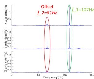
Figure 6: A sample of frequency offset.
