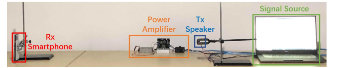
Figure 14: Experimental setup.
