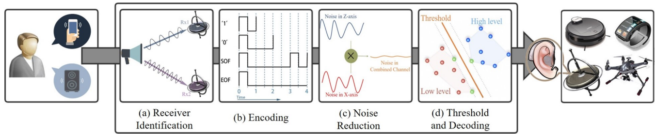
Figure 5: Deaf-Aid , a speaker-to-gyroscope channel for mobile IoT communication, where the transmitter is realized by a smartphone or a commercial speaker and the receiver can be any IoT device equipped with a gyroscope.
