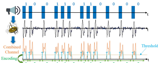
Figure 11: An example of signal transmission.
